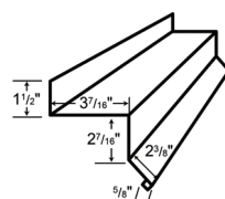
LG 148 "F" CHANNEL
